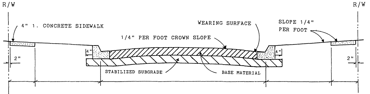
CURB SECTION
