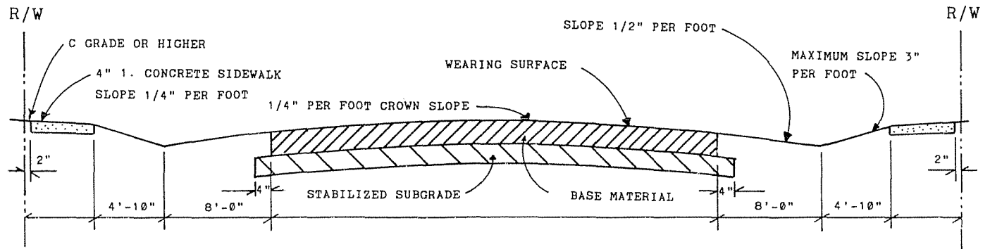
SWALE SECTION
