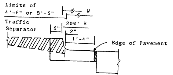
TYPE F CURB AND GUTTER
