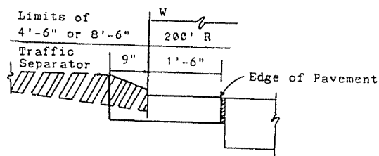
TYPE E CURB AND GUTTER
